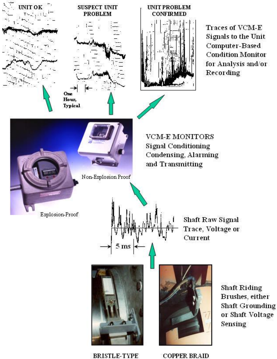
Figure 10 – Unit Condition Monitoring with the VCM-E Warns of Developing Train or Unit Problems
