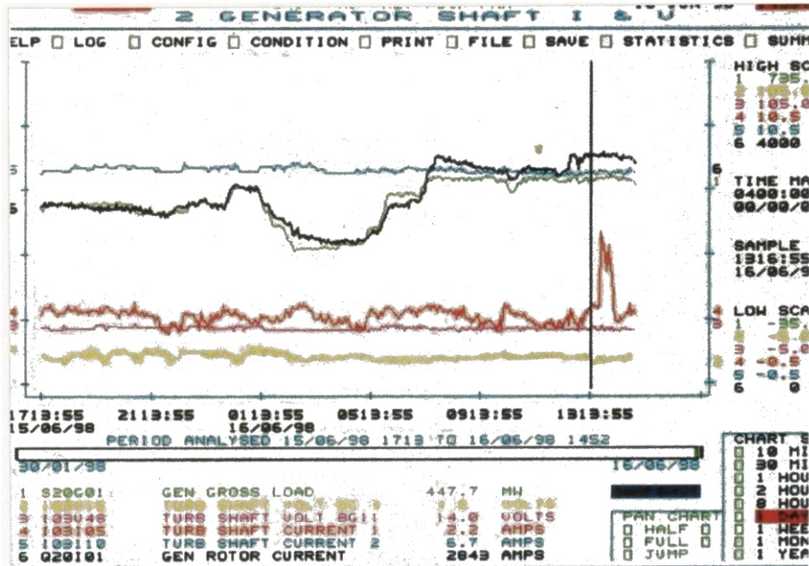
Figure 13 Unit 2 Shaft Peak Currents and Voltages for One Day Grounding brush Currents = 2.2 and 6.7 Amperes Generator OB End Shaft Voltage = 14.0 Volts Turbine Shaft Voltage = 4.8 Volts
