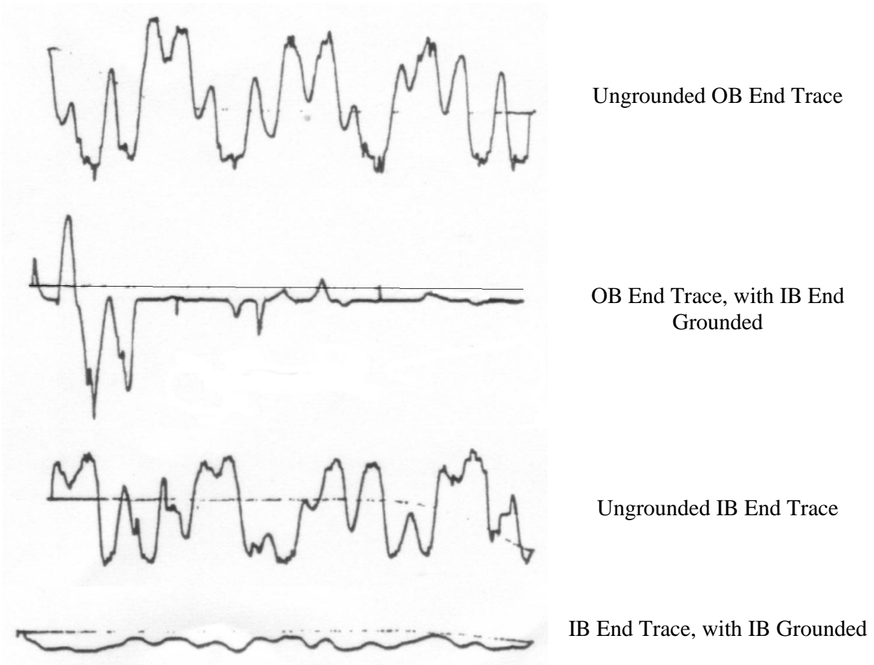
Figure 6 – Erratic Voltages on Shaft Grounding of a Blower Motor
