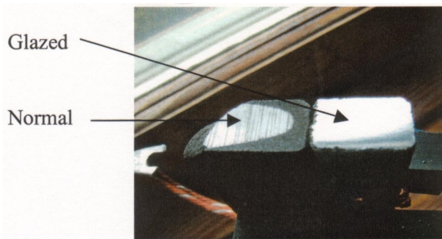
Figure 4 – Carbon Brush Contact Surface Comparison
