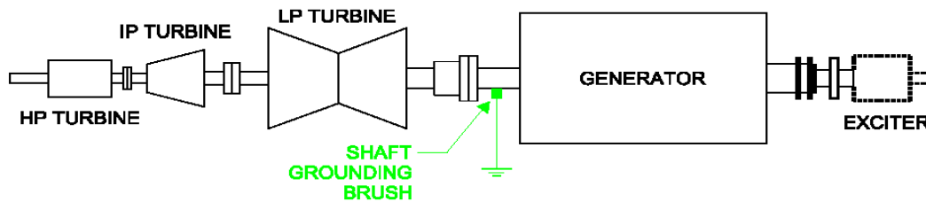
Figure 2 - Shaft Grounding, No Monitor, Possible Protection
