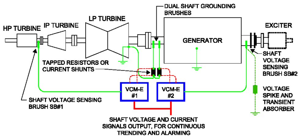
Figure 3 - Shaft Grounding, Monitoring, Protection and Warning
