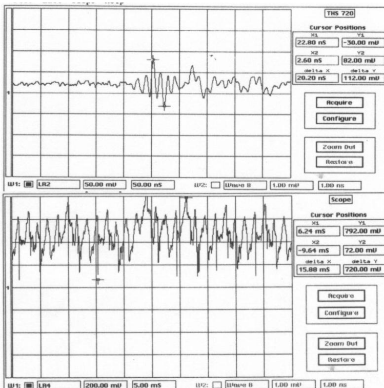
Figure 5 – Comparison of Traces with Different Time Scaling
