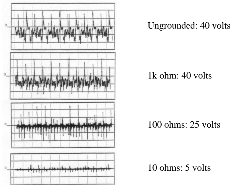
Figure 8 – Shaft Electromagnetic voltages with Different Resistances in the Shaft Grounding Circuit
