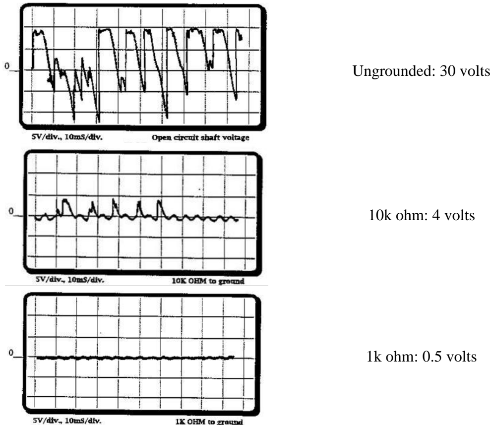
Figure 9 – Shaft Electrostatic Voltages with Different Resistances in the Shaft Grounding Circuit
