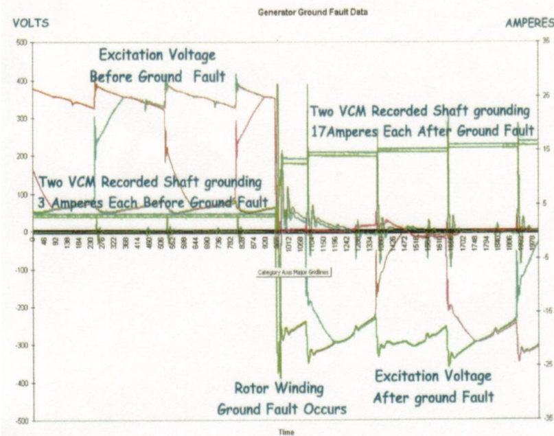
Figure 14 - 500 MW Turbine Generator Field Voltage Shift and Shaft Grounding Current Increase (Left) During a Rotor Excitation Winding Ground Fault (Right)
