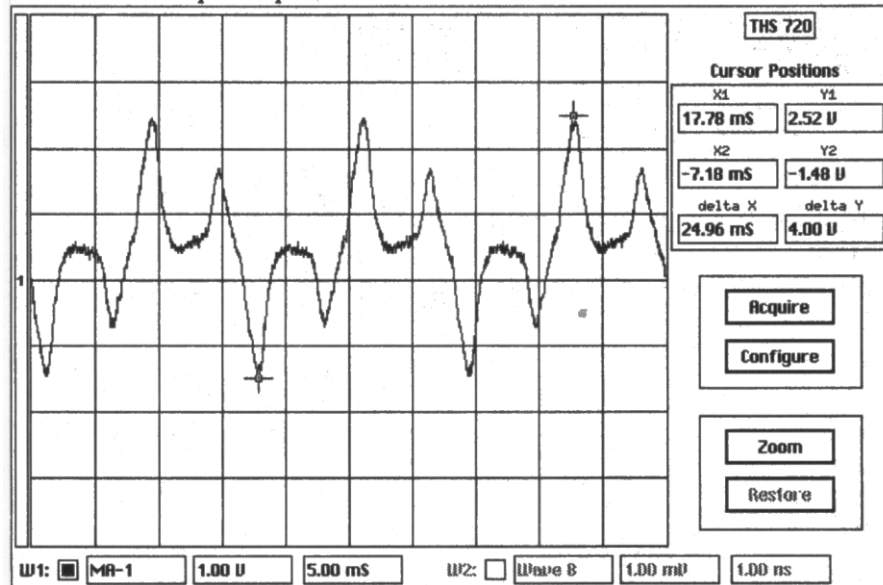
Figure 7 – Grounding Current Oscilloscope Trace at 60 Hz, Plus a Strong Common-Mode Third Harmonic
