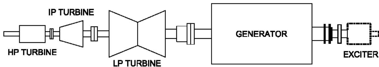
Figure 1 - No Brushes, No Monitors and No Protection
